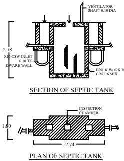
SEPTIC TANK
