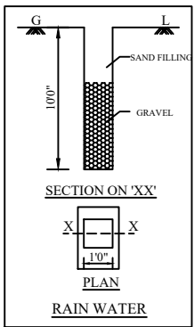
RAINWATER HARVESTING
