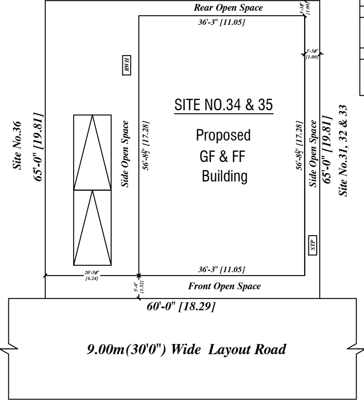
Site Plan
