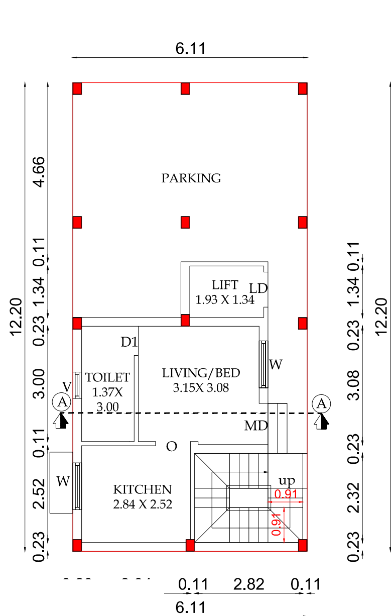
FLOOR PLAN
