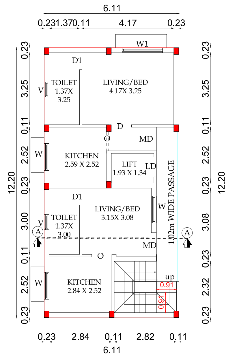
TYPICAL FIRST AND SECOND FLOOR PLAN
