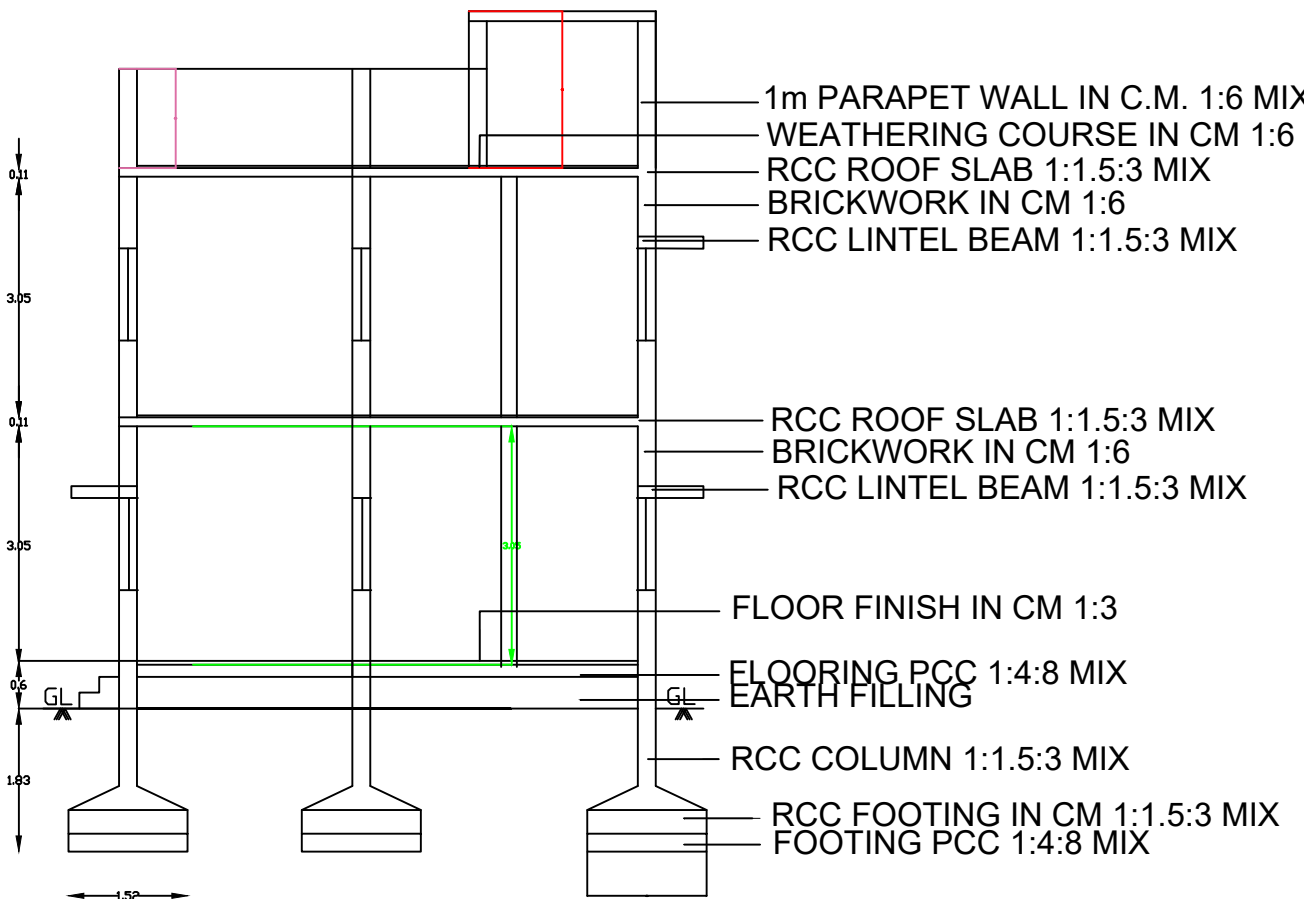
CROSS SECTION ON XY
