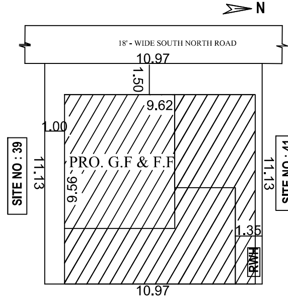
SITE NO: 27 SITE PLAN
