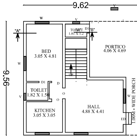
PRO. GROUND FLOOR
