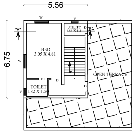
PRO. FIRST FLOOR
