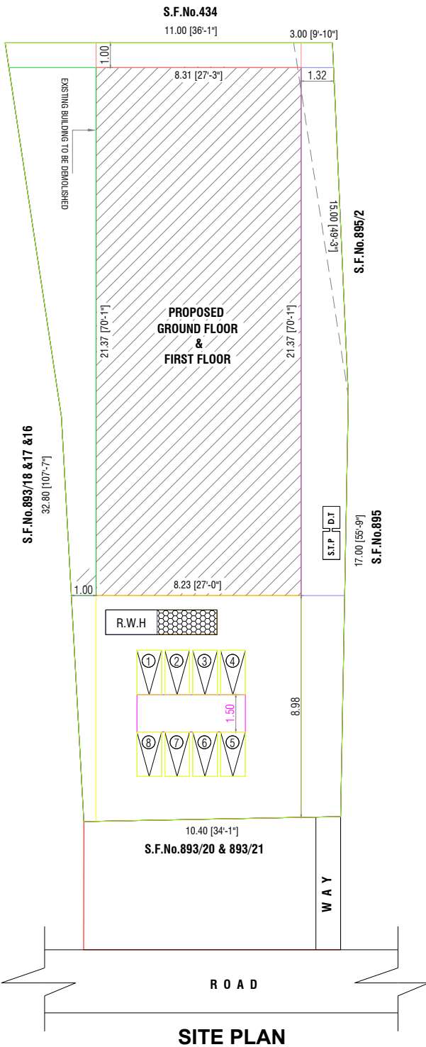
SITE PLAN
