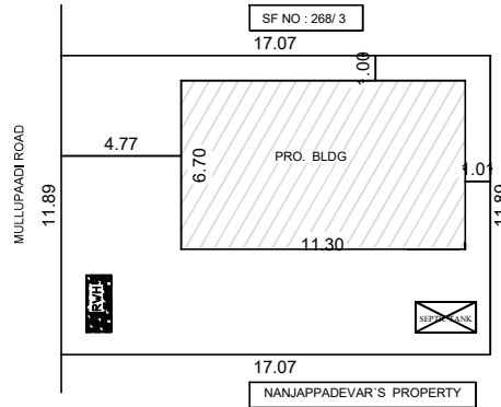
SITE PLAN
