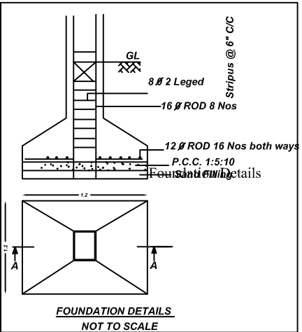
FOUNDATION DETAILS NOT TO SCALE
