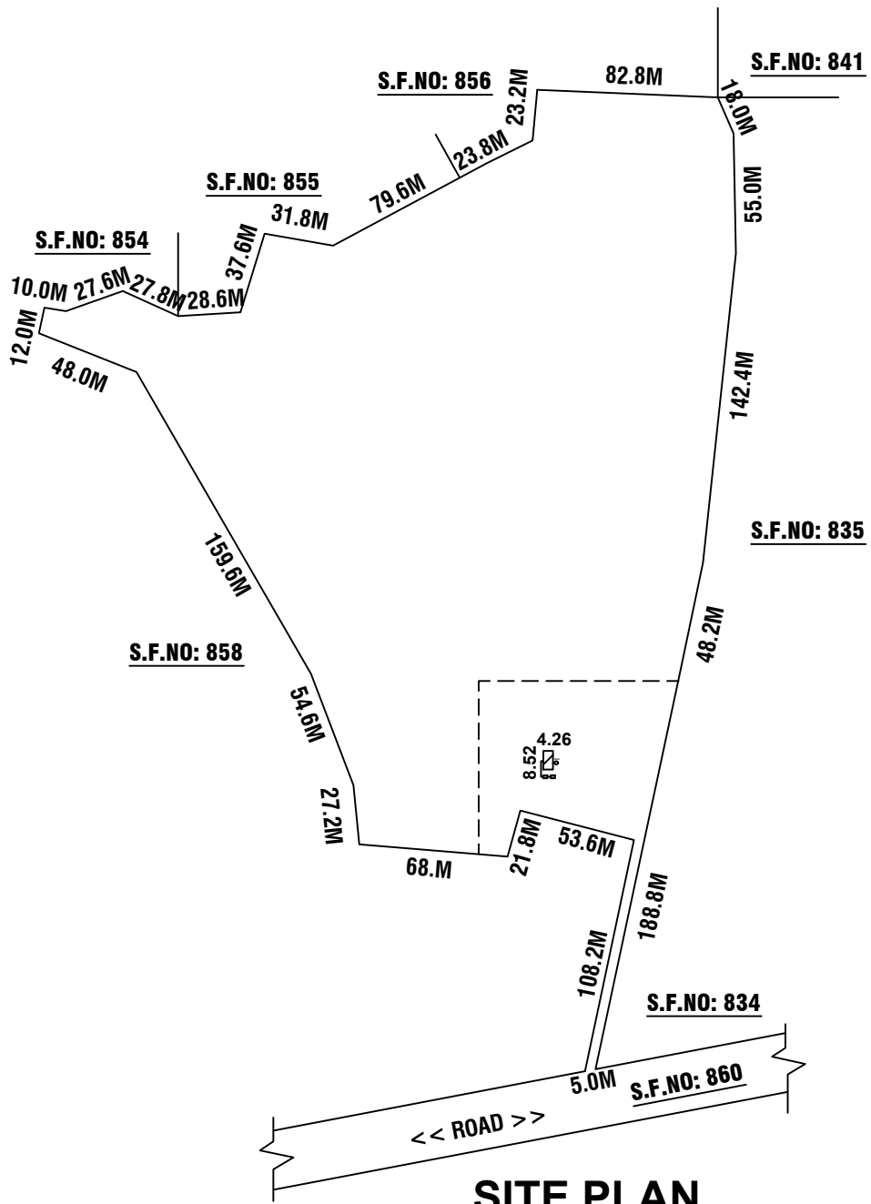
SITE PLAN
