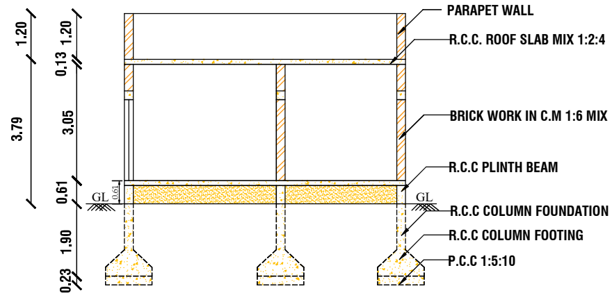
CROSS SECTION AT A-A
