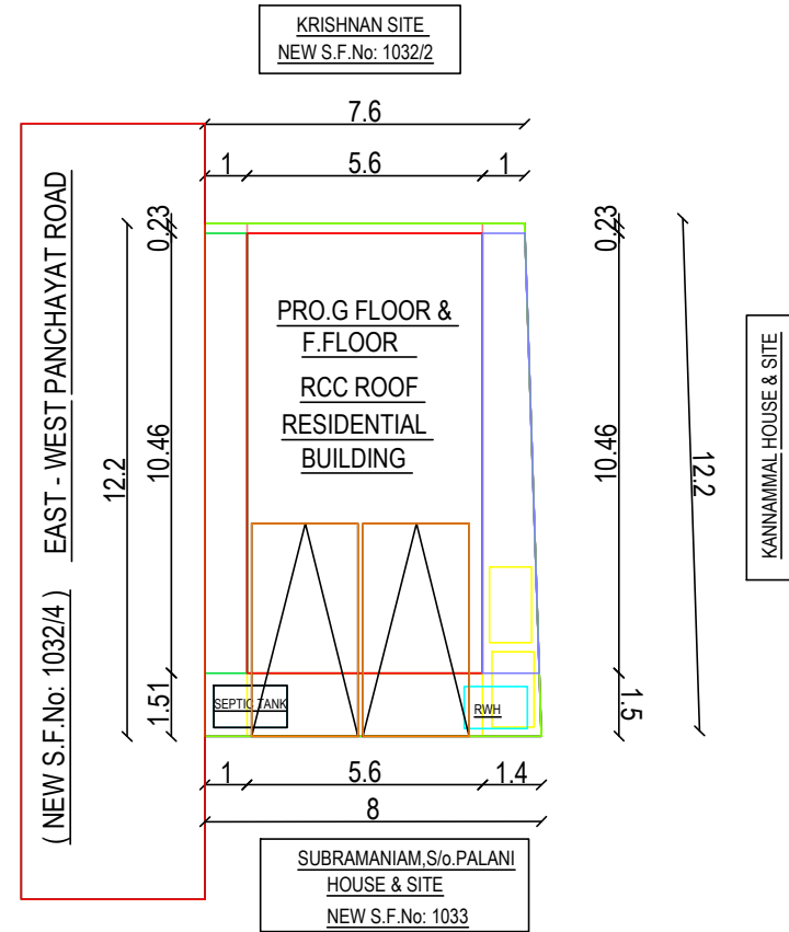
SITE PLAN
