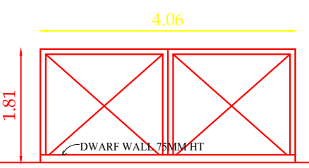
MAIN GATE ELEVATION
