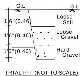
TRIAL PIT (NOT TO SCALE)
