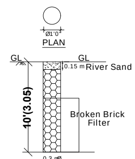
SECTION OF THE PERCOLATION PIT (NOT TO SCALE)
