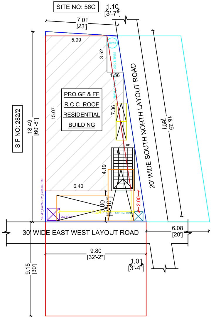
SITE PLAN
