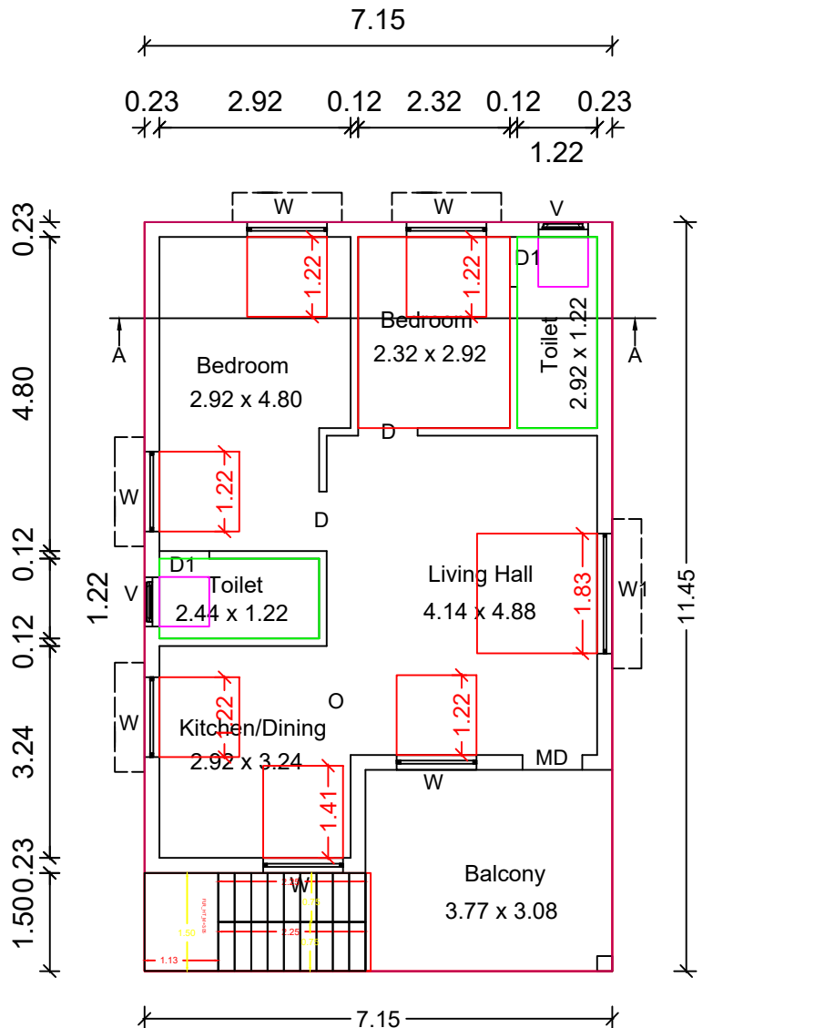
PRO. ADDITIONAL FIRST FLOOR PLAN
