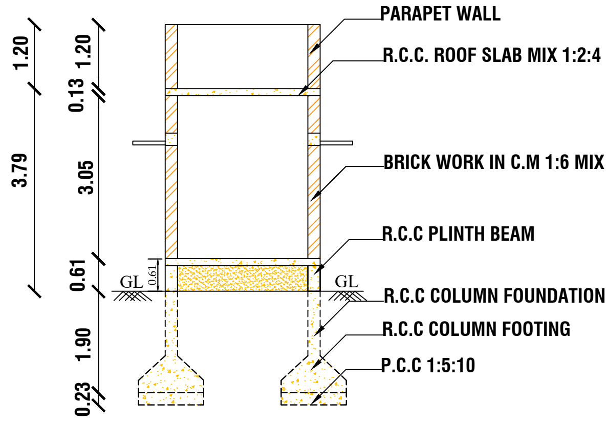
CROSS SECTION AT A-A
