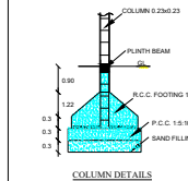
COLUMN DETAILS
