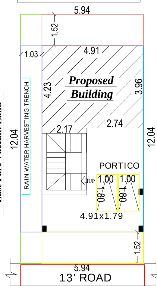
SITE PLAN
