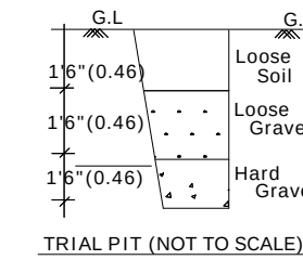
TRIAL PIT (NOT TO SCALE)
