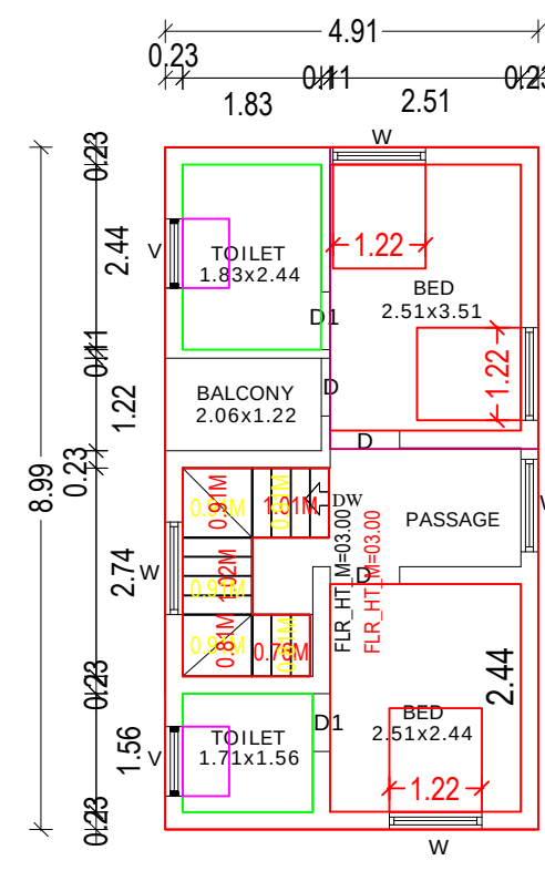
SECOUND FLOOR
