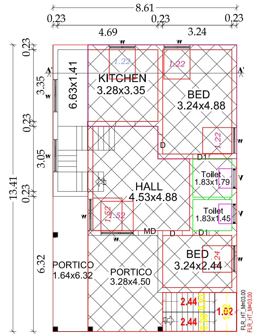
EXG. AND PRO. ADD. GROUND FLOOR PLAN
