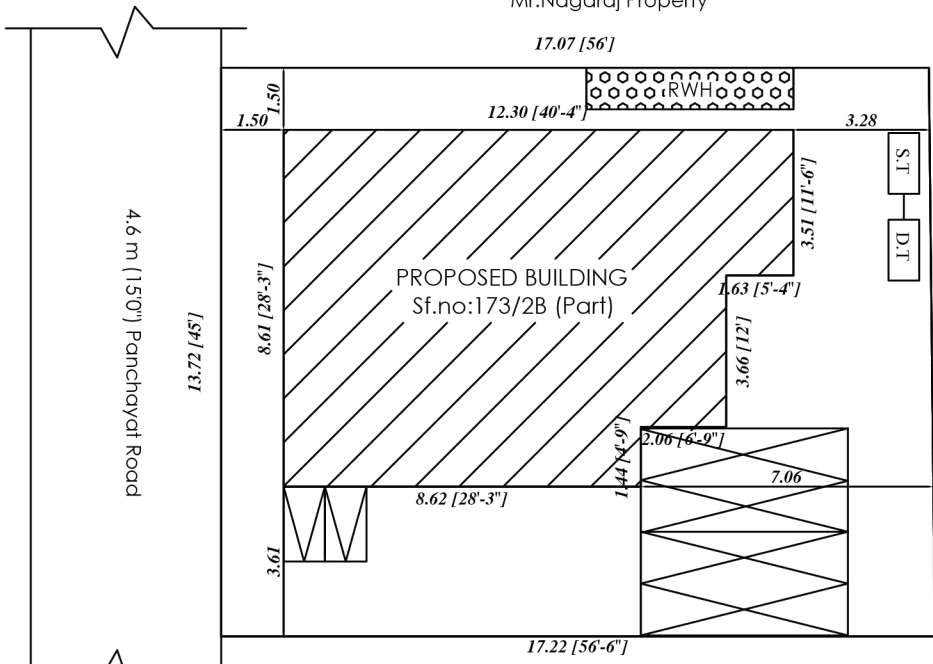
Site Plan
