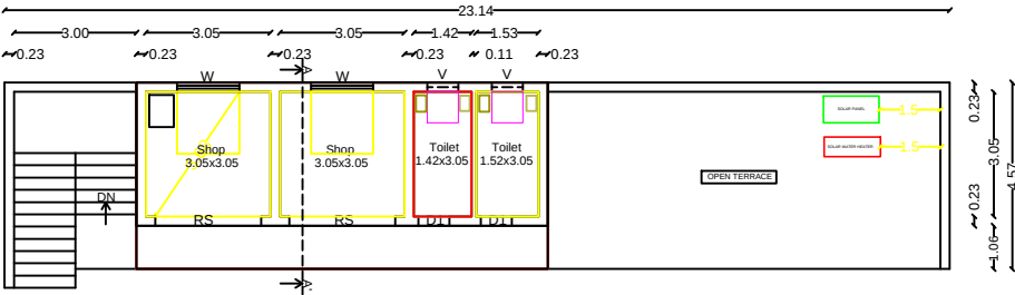
PROPOSED FIRST FLOOR PLAN SCALE 1:100
