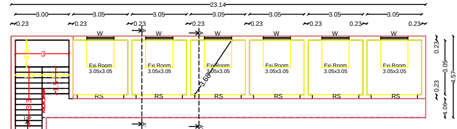
EXISTING & ADDITIONAL GROUND FLOOR PLAN SCALE 1:100
