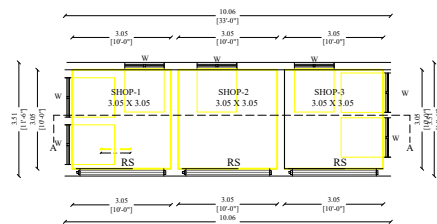
PROPOSED GROUND FLOOR PLAN
