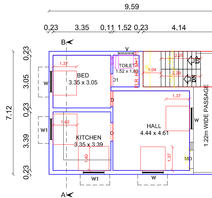
PRO.ADDL.FIRST FLOOR PLAN
