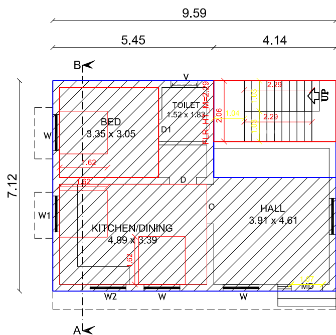
EXISTING & PRO.ADDL.GROUND FLOOR PLAN
