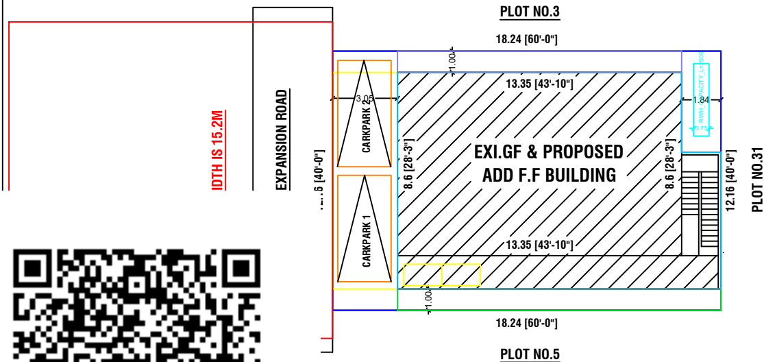
SITE PLAN
