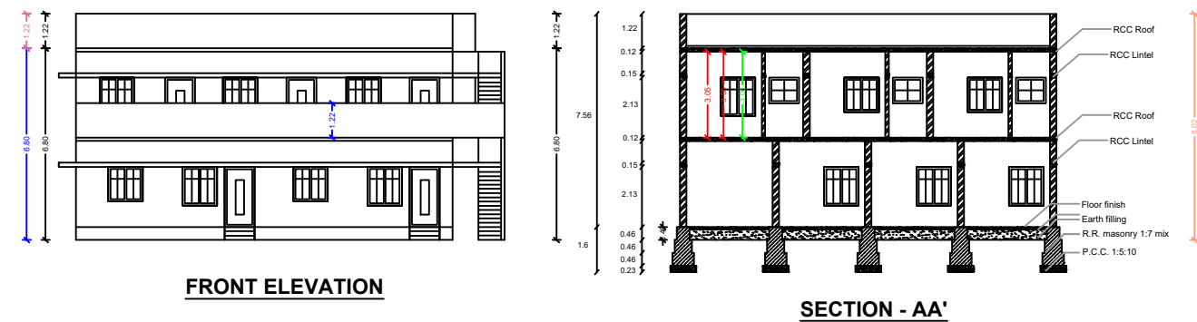
SECTION - AA'
