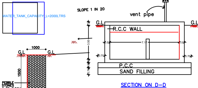
SECTION ON D-D
