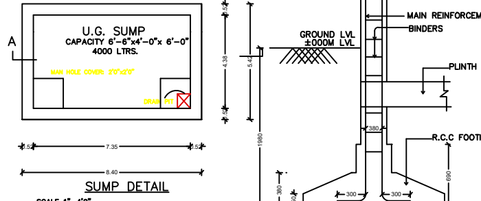
SUMP DETAIL
