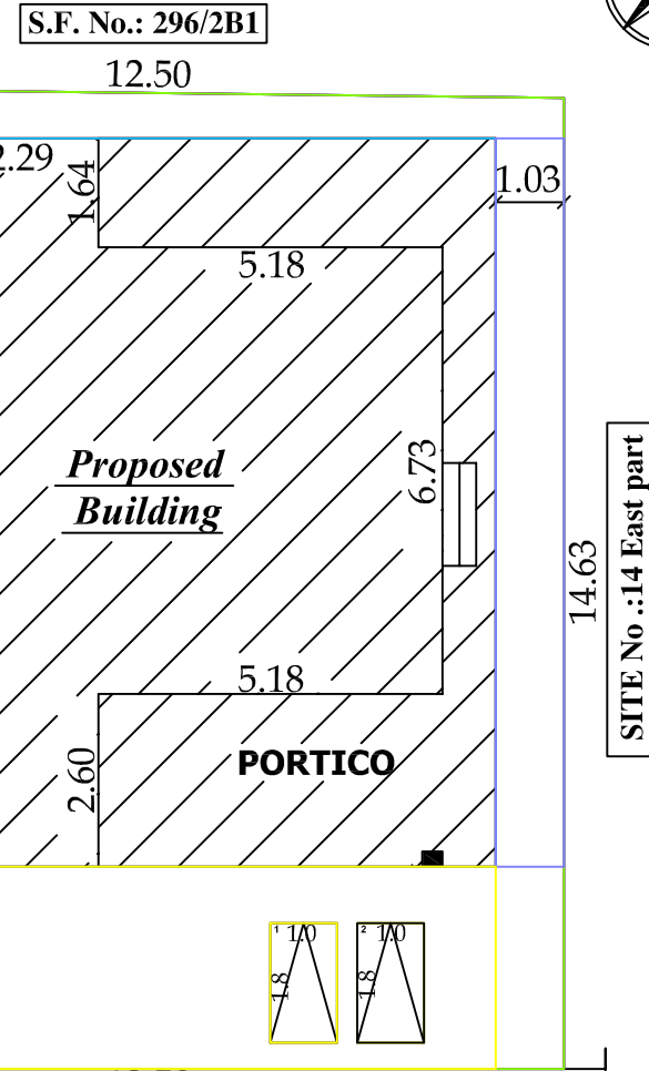
SITE PLAN
