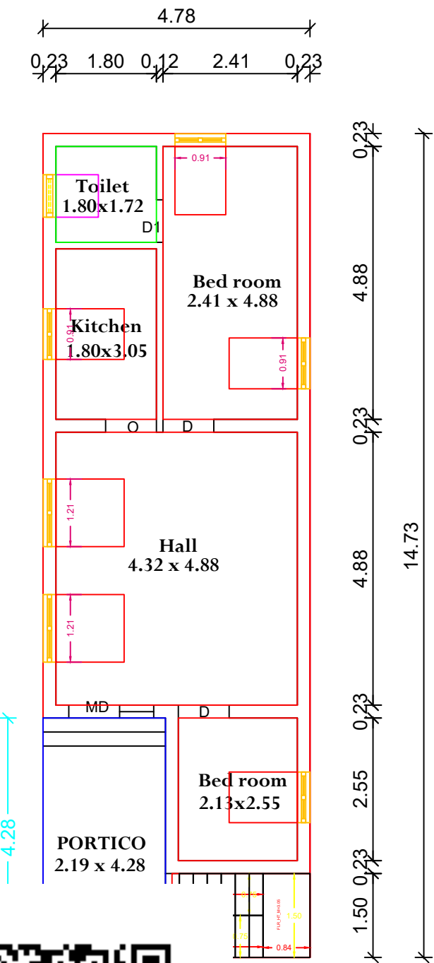
FLOOR PLAN
