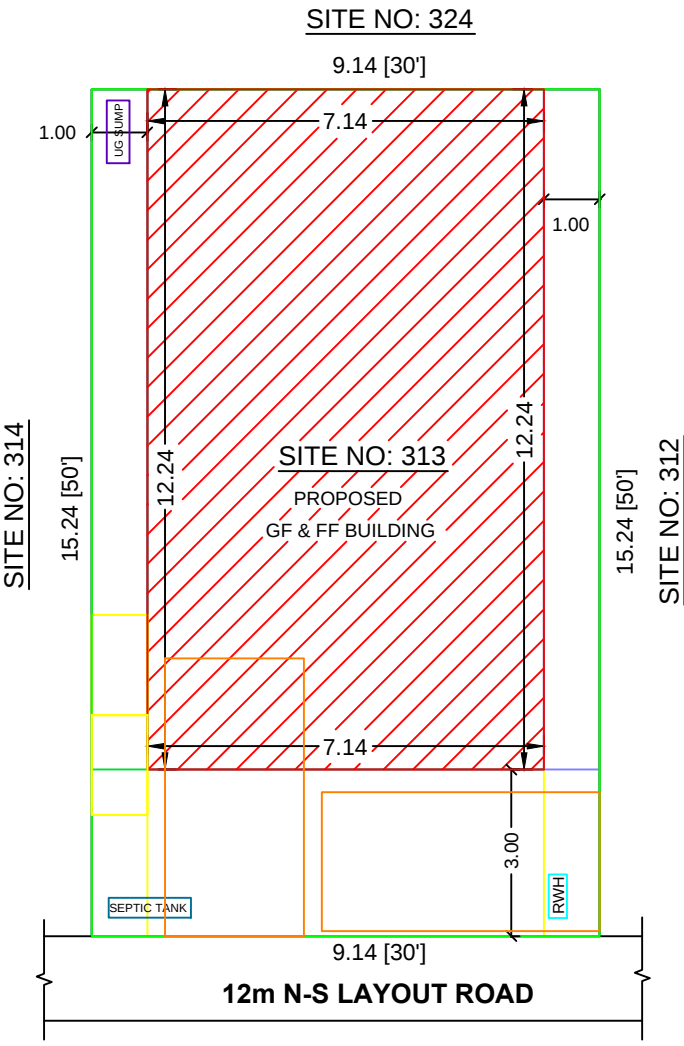
SITE PLAN
