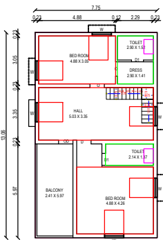
PROPOSED FIRST FLOOR BUILDING
