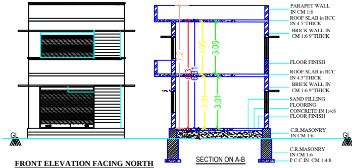
FRONT ELEVATION FACING NORTH
