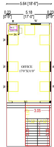
PROPOSED FIRST FLOOR
