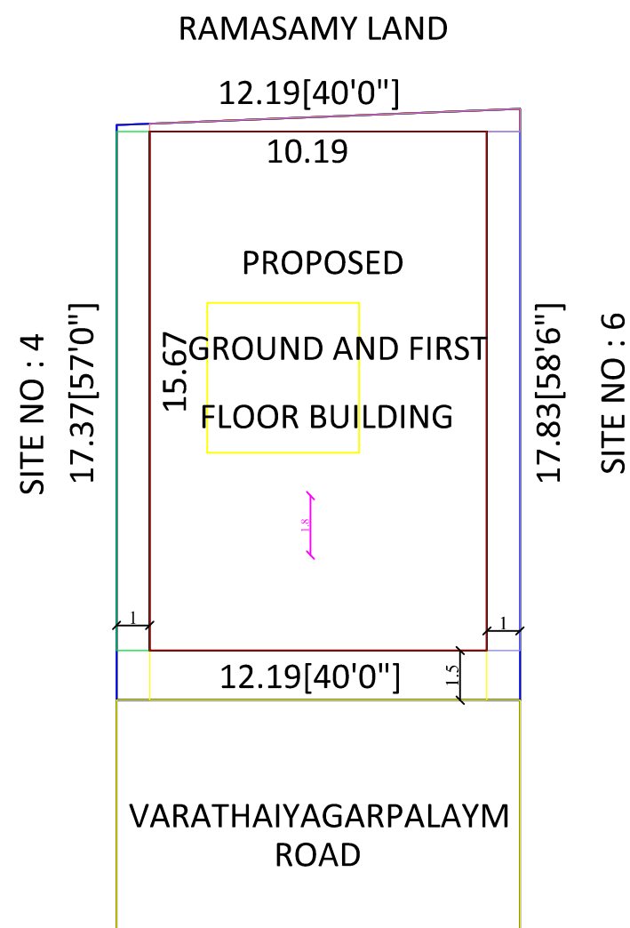
SITE PLAN
