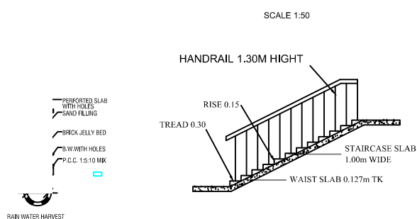
STAIRCASE DETAILS
