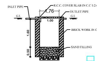
SECTIONAL DETAILS
