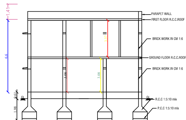
SECTION AB
