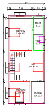
PROPOSED FIRST FLOOR BUILDING
