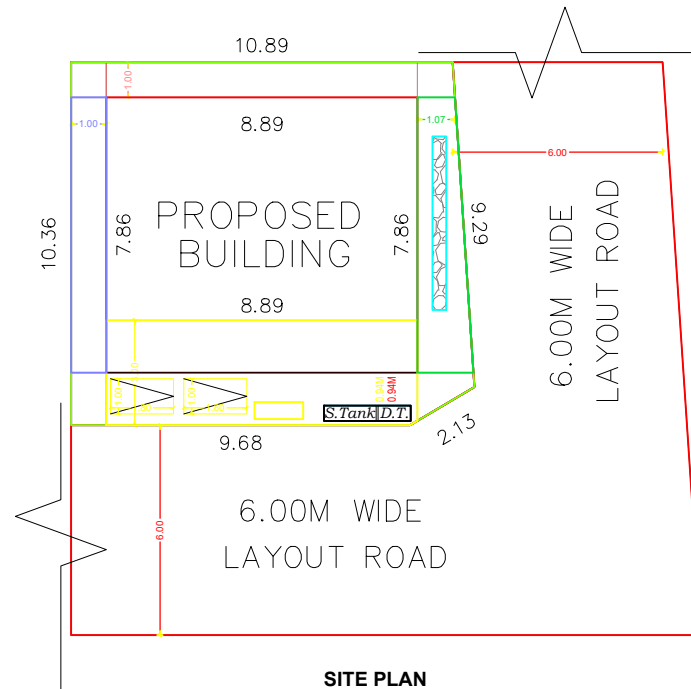
SITE PLAN
