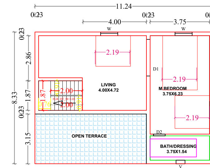
PROPOSED SECOND FLOOR
