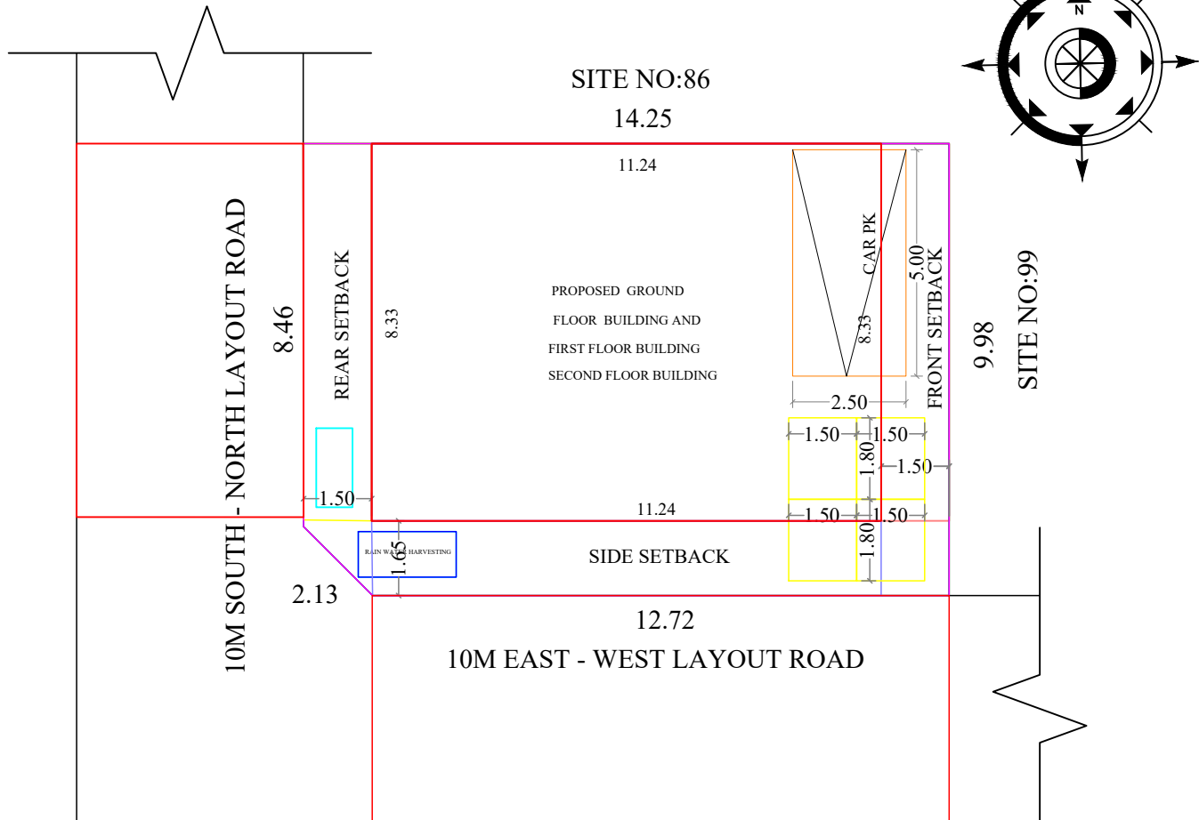
SITE PLAN
