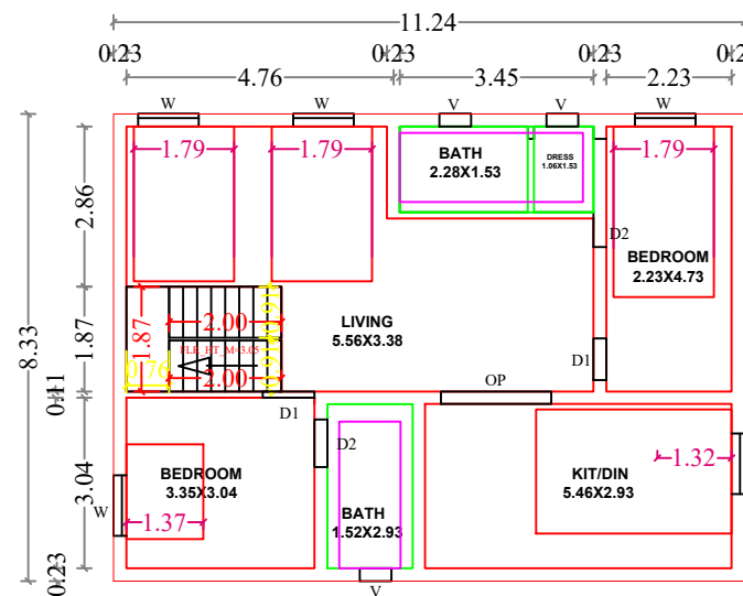
PROPOSED FIRST FLOOR
