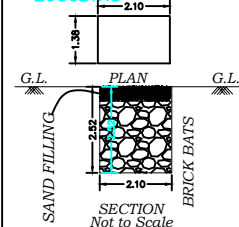
SECTION Not to Scale
