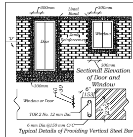
Typical Details of Providing Vertical Steel Bars
