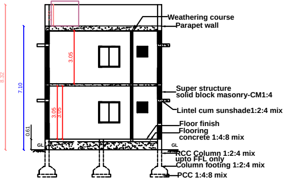
SECTION ELEVATION
