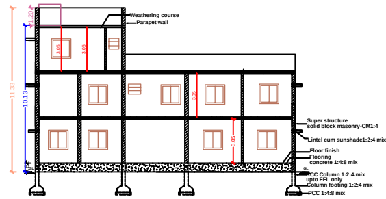
SECTION ELEVATION
