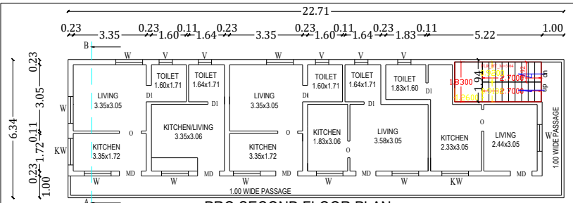
PRO. SECOND FLOOR PLAN (RESIDENTIAL)
