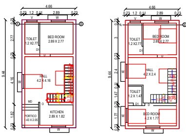
PROPOSED GROUND FLOOR BUILDING PROPOSED FIRST FLOOR BUILDING
