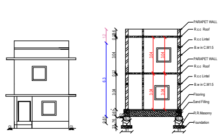
ELEVATION SECTION ON "AB"
