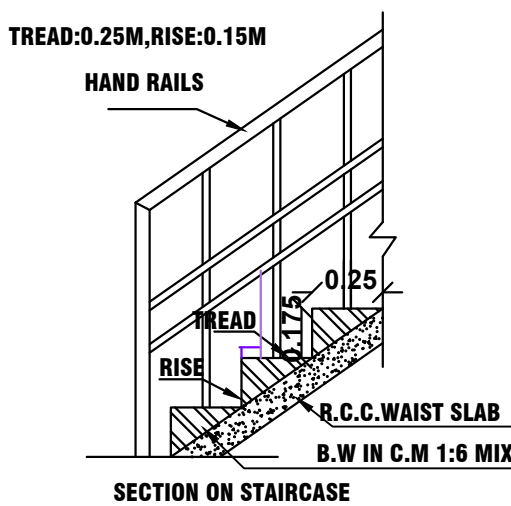
SECTION ON STAIRCASE
