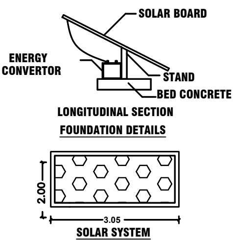
SOLAR SYSTEM
