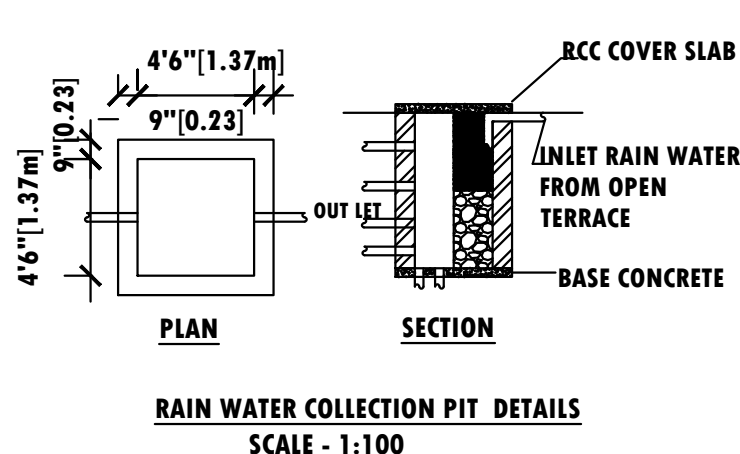
RAIN WATER COLLECTION PIT DETAILS SCALE - 1:100
