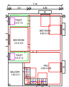
PROPOSED FIRST FLOOR BUILDING
