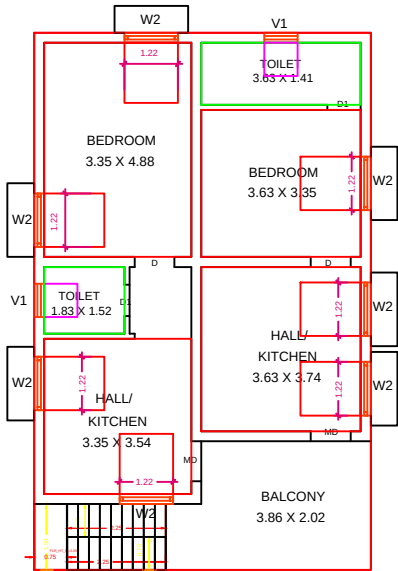
PRO. SECOND FLOOR PLAN
