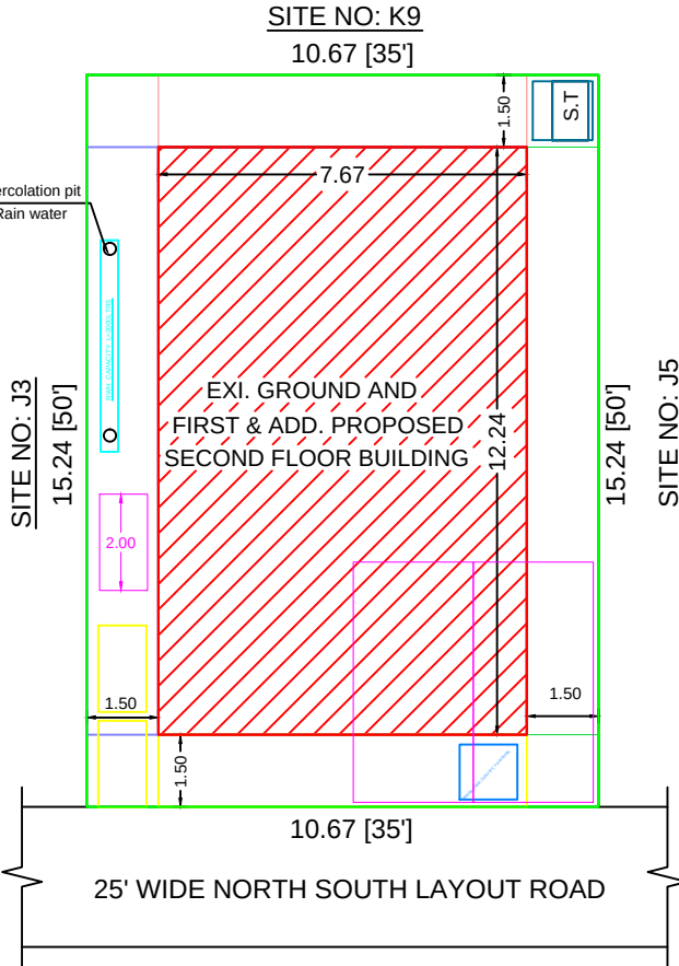
SITE PLAN
