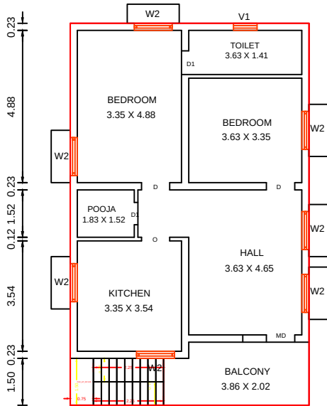
EXI. FIRST FLOOR PLAN
