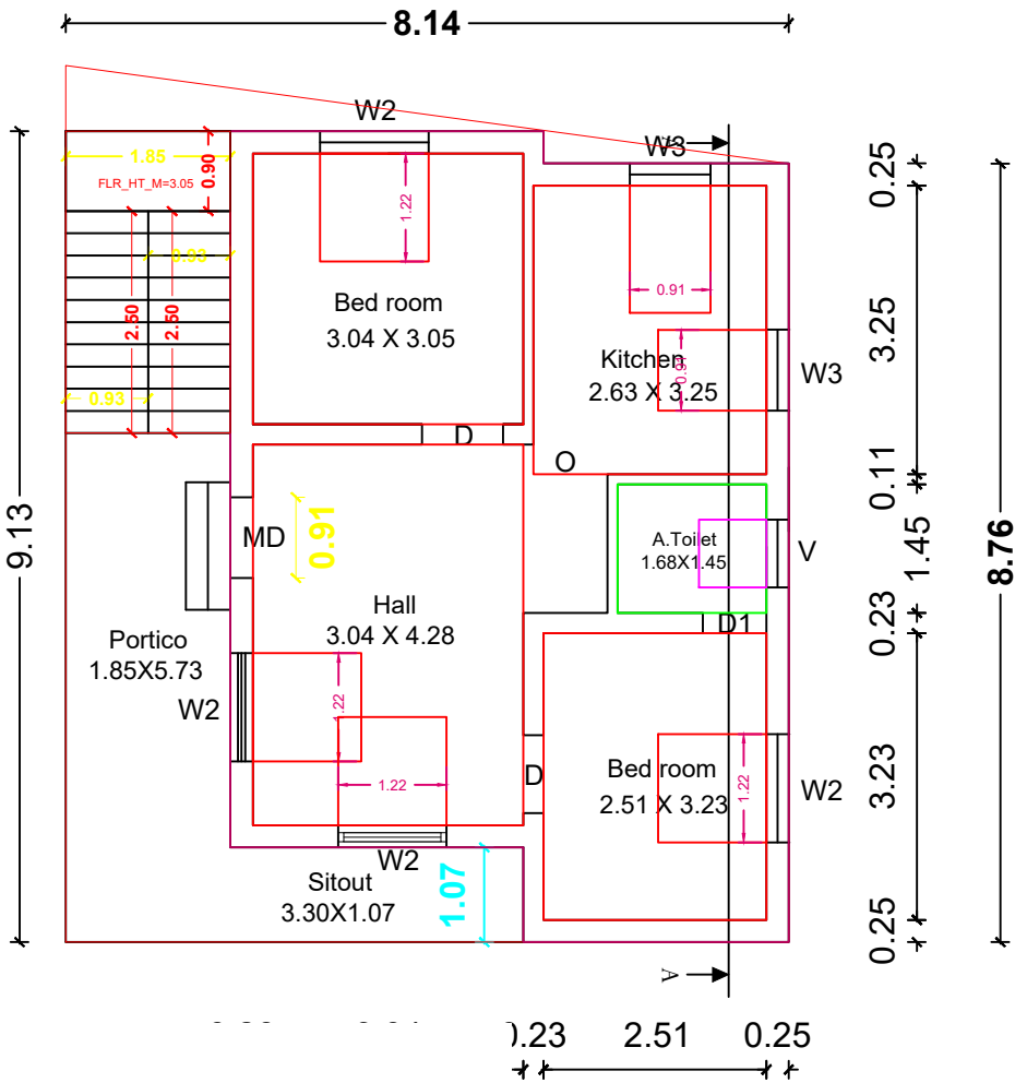
JD FLOOR PLAN
