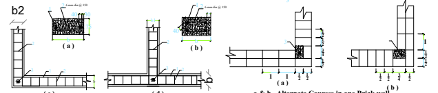
Figure - 2 : Typical Details of Providing Vertical Steel Bars in Brick Masonry.
