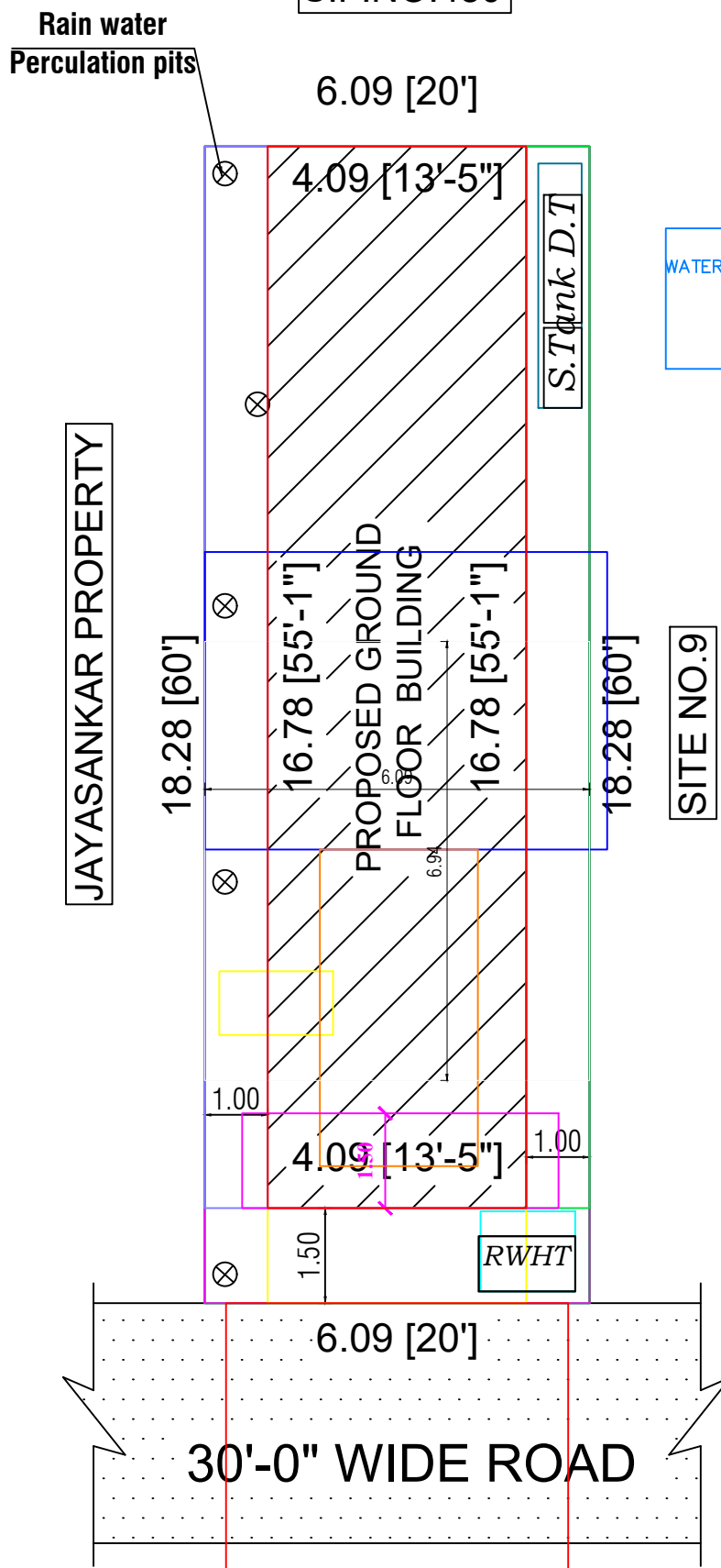
SITE PLAN
