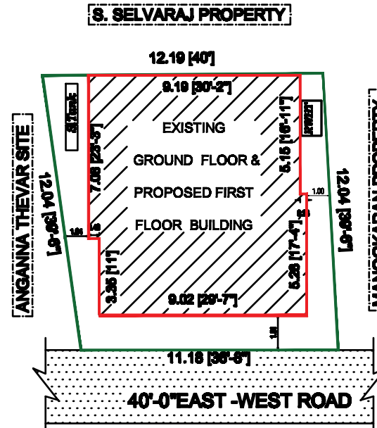
SITE PLAN
