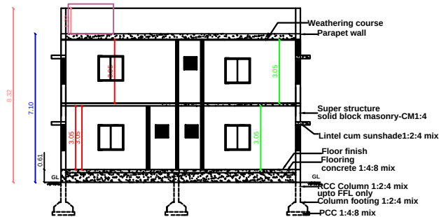
SECTION ELEVATION
