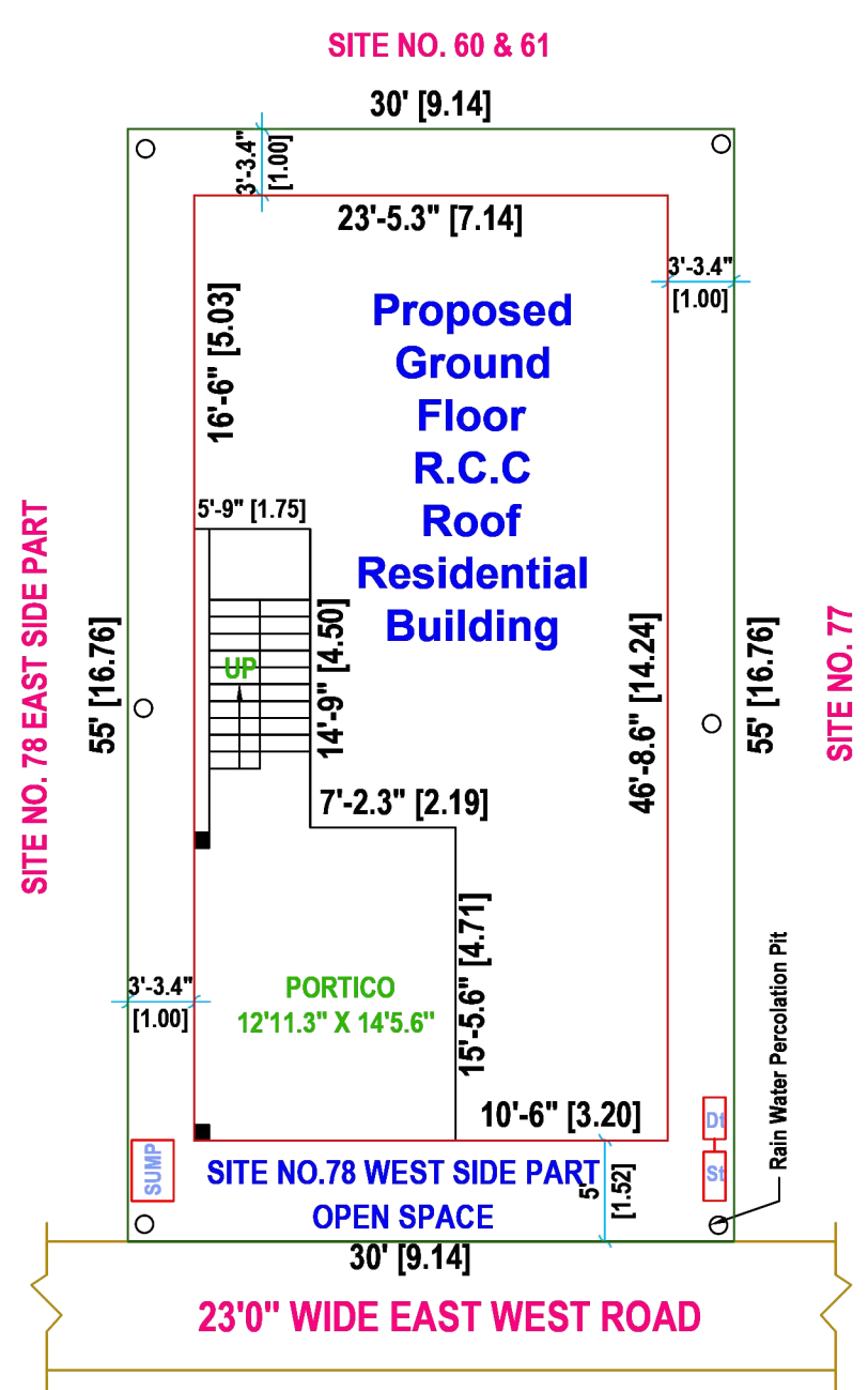
SITE PLAN (SCALE - 1" : 8' 0")
