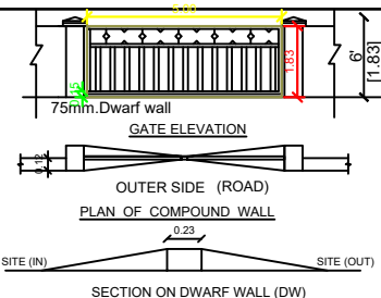
SECTION ON DWARF WALL (DW)
