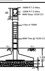
RCC COLUMN DETAILS
