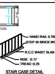
STAIR CASE DETAIL
