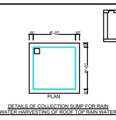
DETAILS OF COLLECTION SUMP FOR RAIN WATER HARVESTING OF ROOF TOP RAIN WATER RWV_CAPACITY_L=5000LTRS
