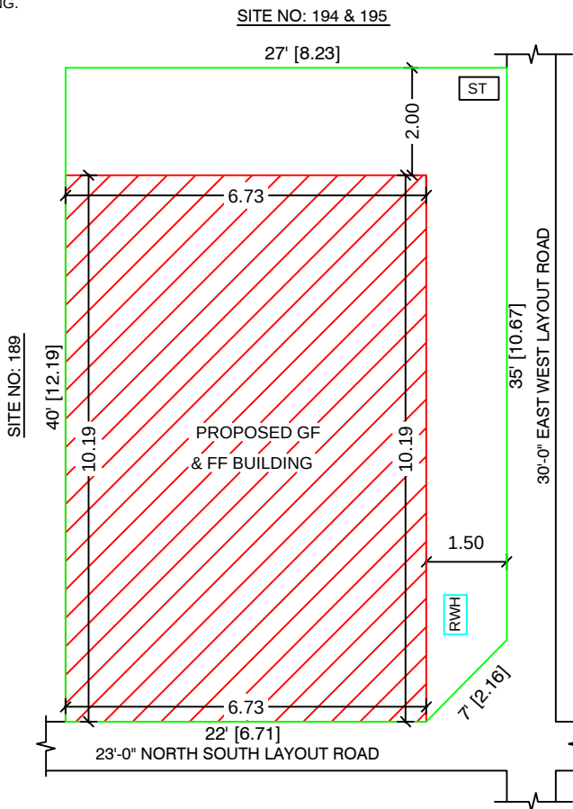
SITE PLAN
