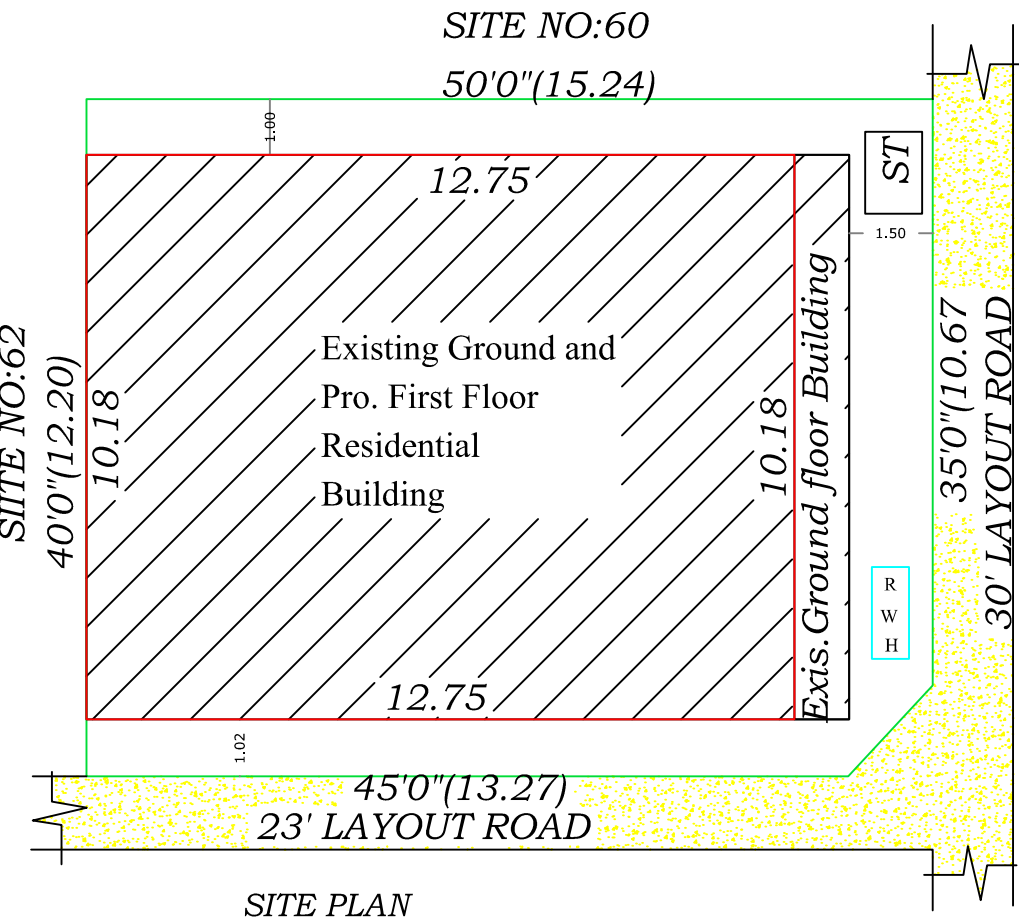
SITE PLAN
